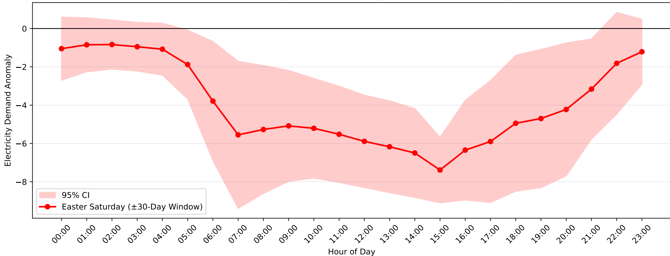
Burwood Demand Anomaly: Easter Saturday (2004-2017, \pm 30 -Day Window)
